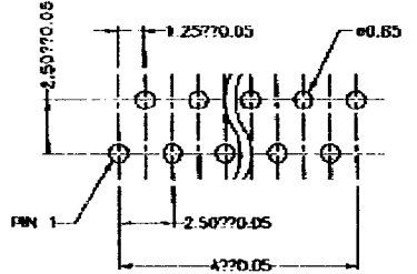
STANDARD PCB LAYOUT
