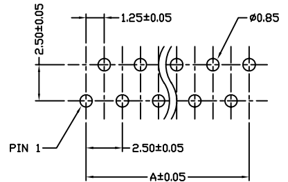
STANDARD PCB LAYOUT
