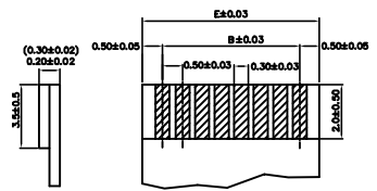
FFC/FPC DIMENSION
