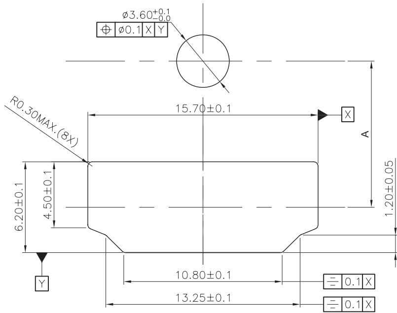
RECOMMENDED PANEL CUT OUT DIMENSION
