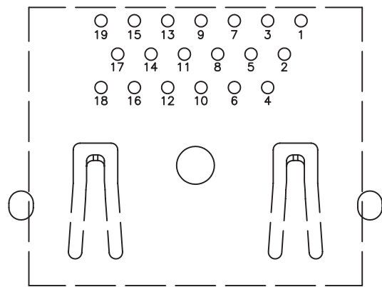
PIN ASSIGNMENT
